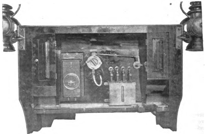
STEEL DASHBOARD OF THOMAS CAR.—TOOL LOCKERS IN UPPER CORNERS. ] 5
